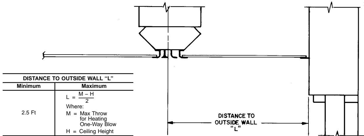
Fig. 8 — Recommended Location for Changeover Moduline® Heating/Cooling
